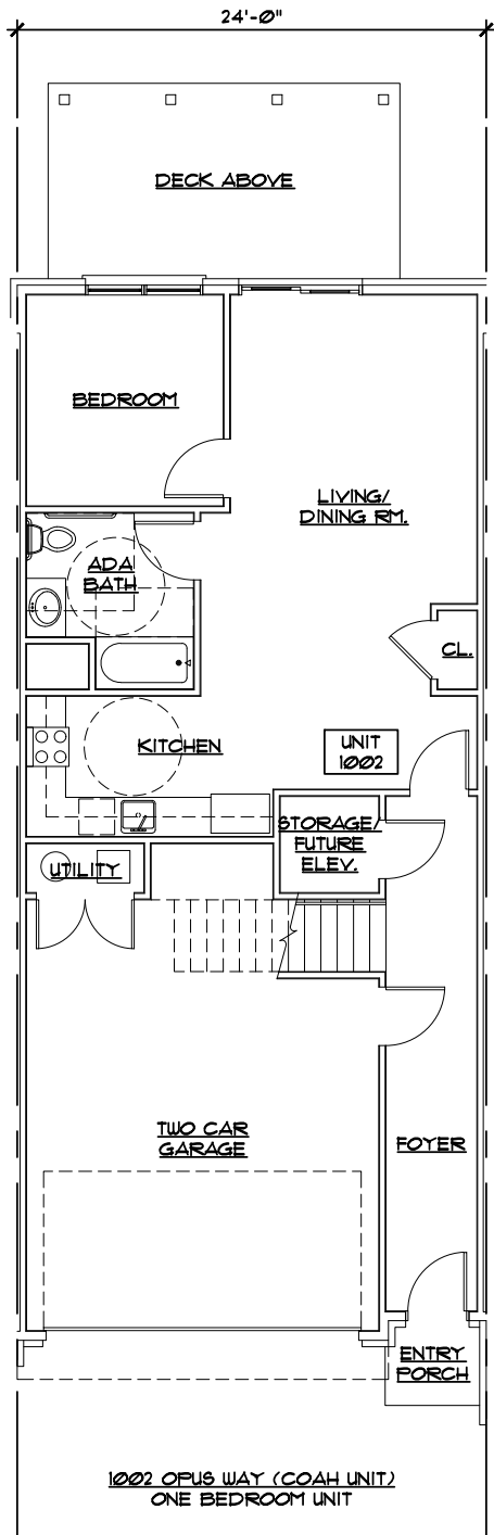
BUILDING 10 FIRST FLOOR PLAN
